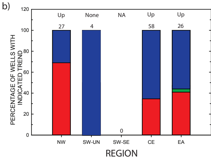
Figure 3: Results of the Regional Kendall analysis for the upper glacial aquifer a) long term (1982-2008), b) short term (1982-1994), and the Magothy aquifer c) long term and d) short term.
